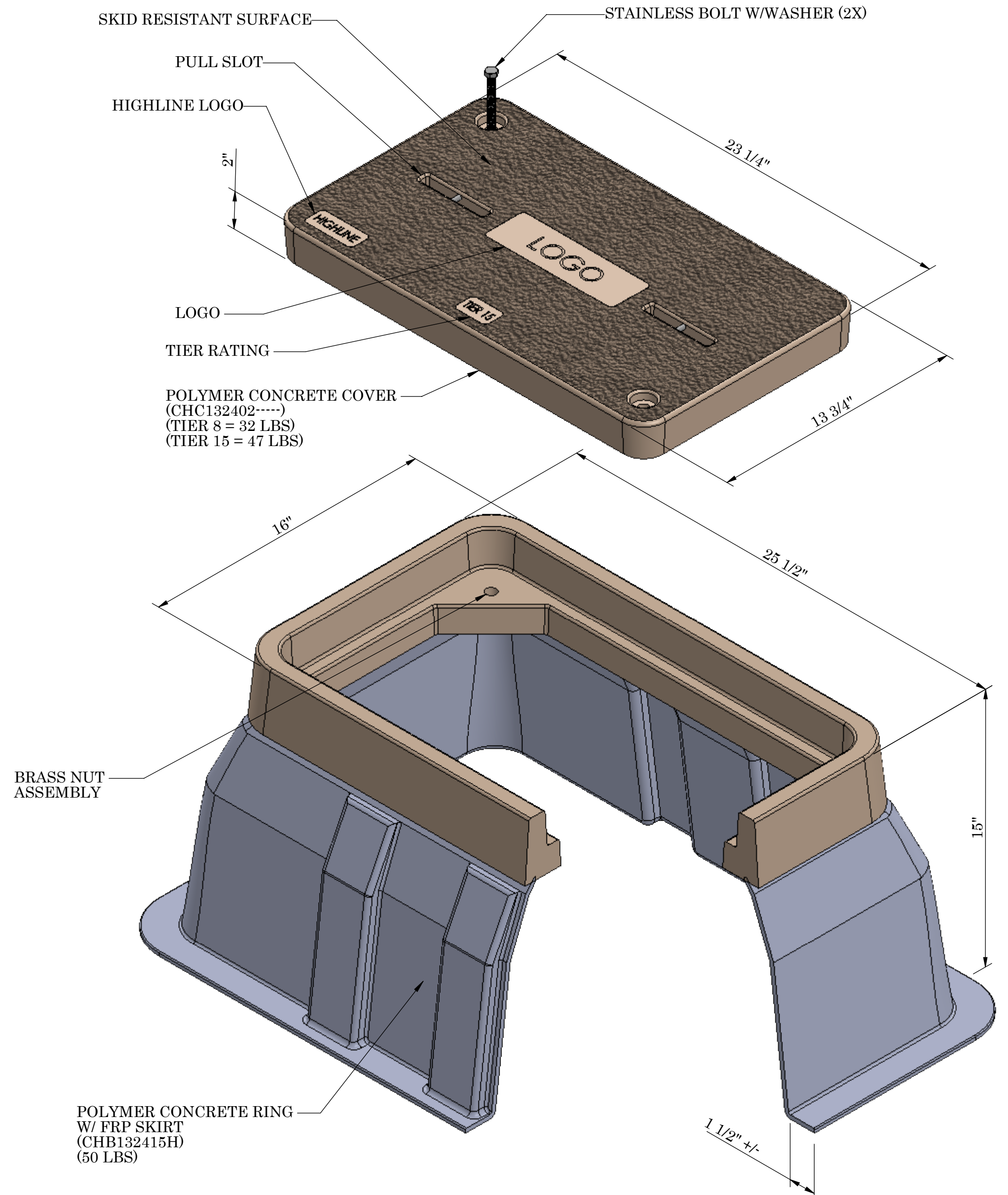
ISOMETRIC VIEW
