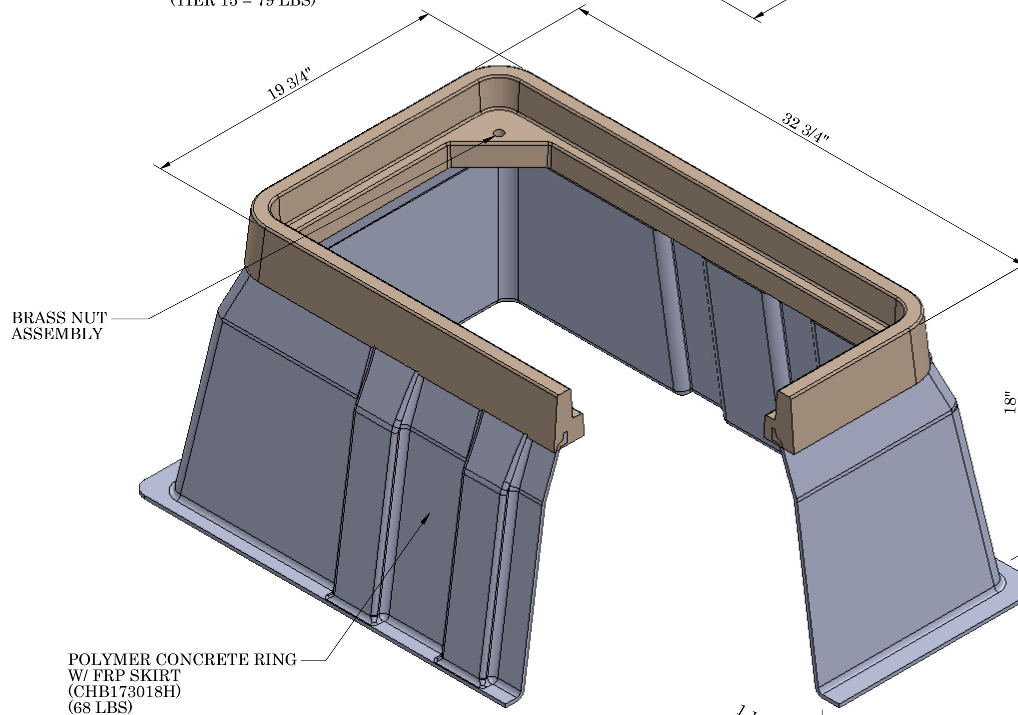
ISOMETRIC VIEW
