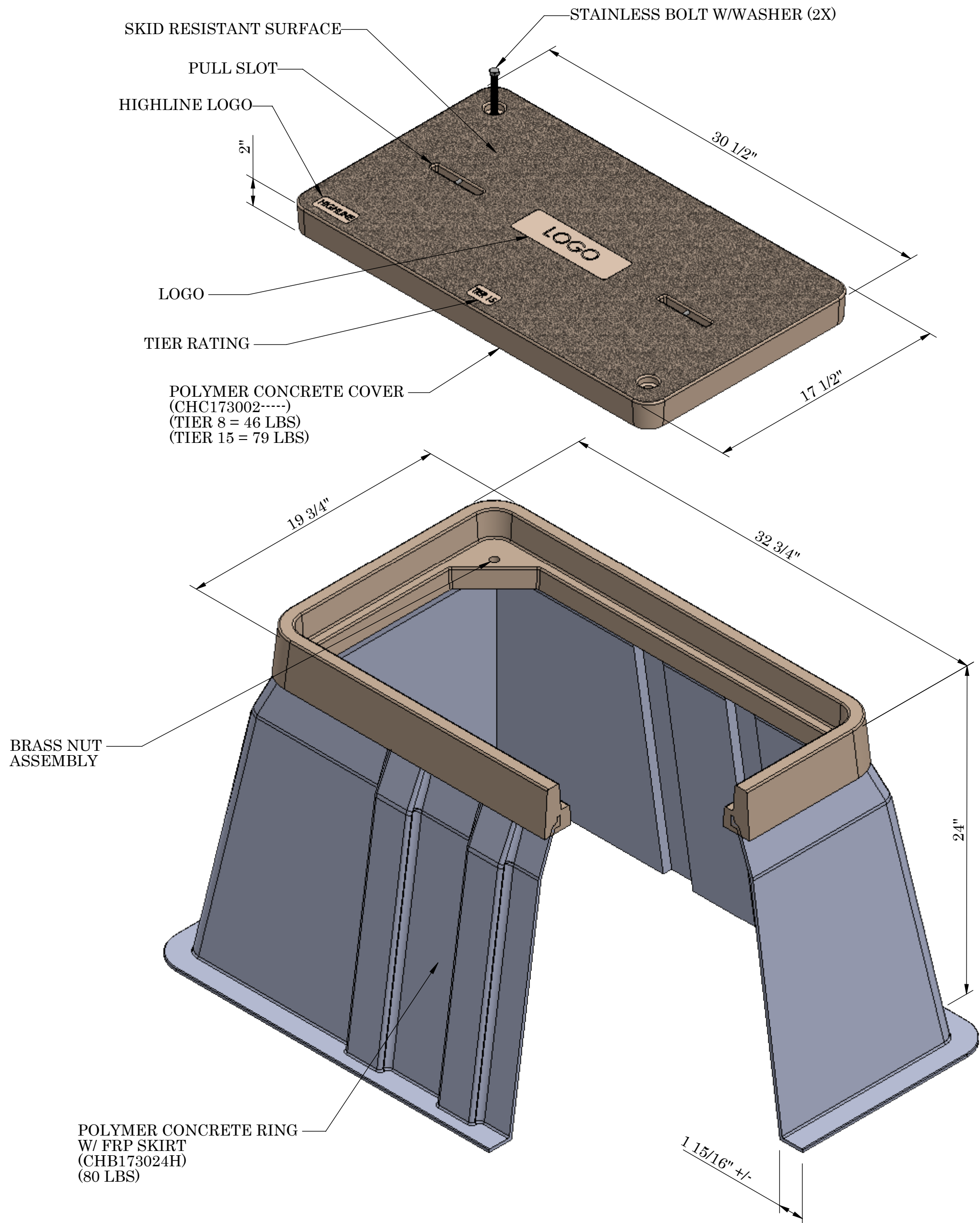
ISOMETRIC VIEW
