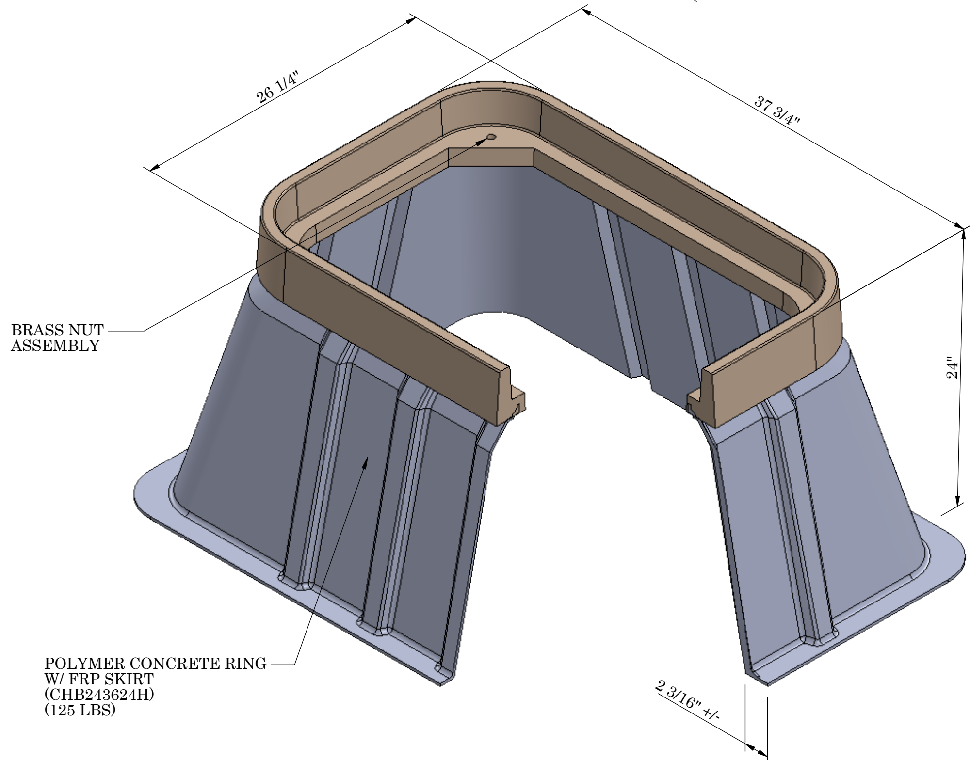
ISOMETRIC VIEW
