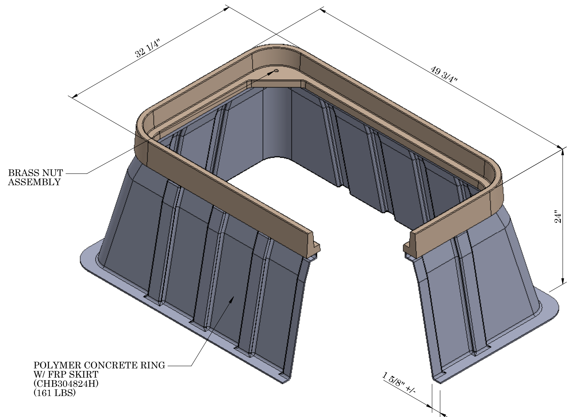
ISOMETRIC VIEW
