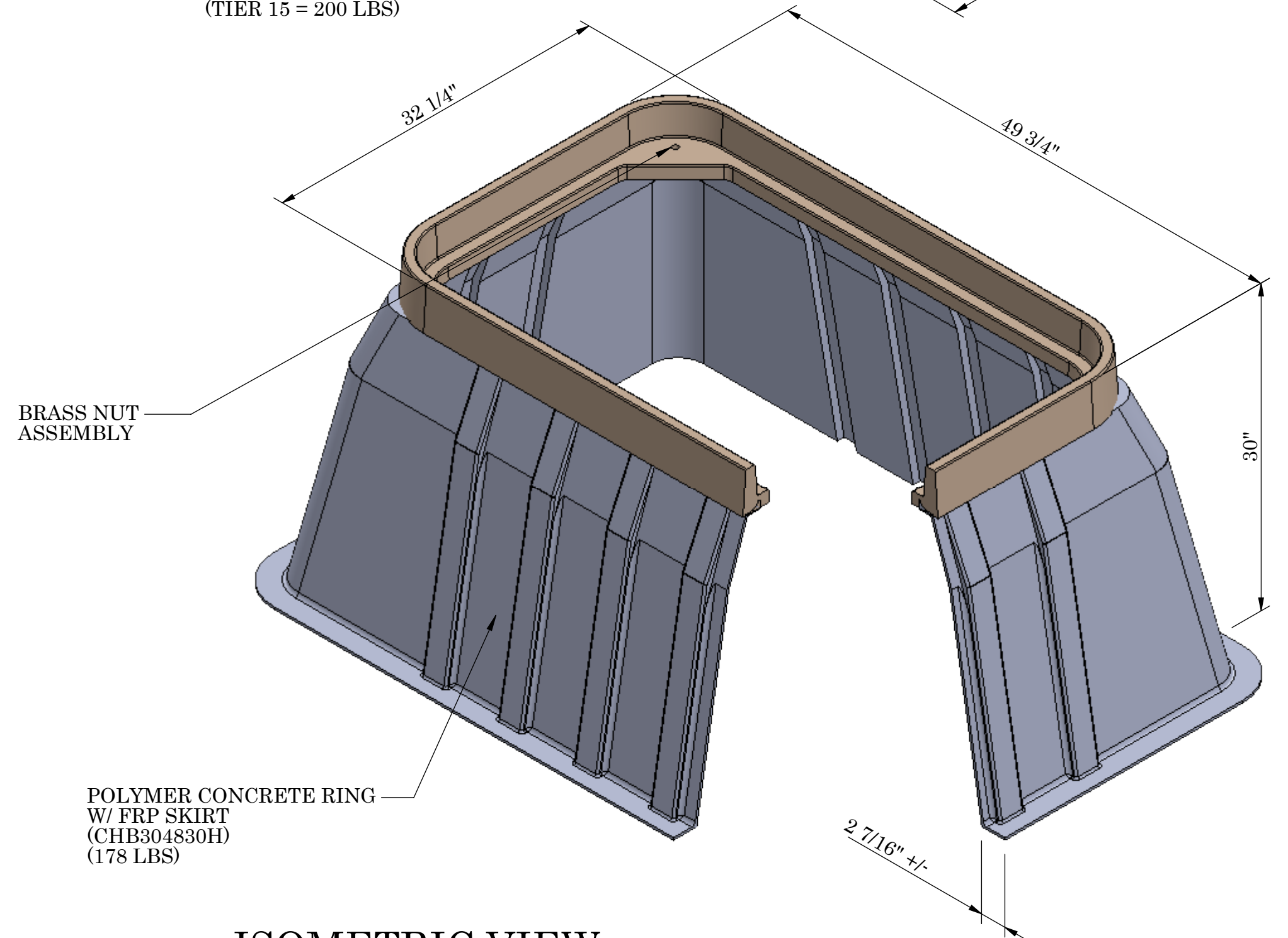
ISOMETRIC VIEW
