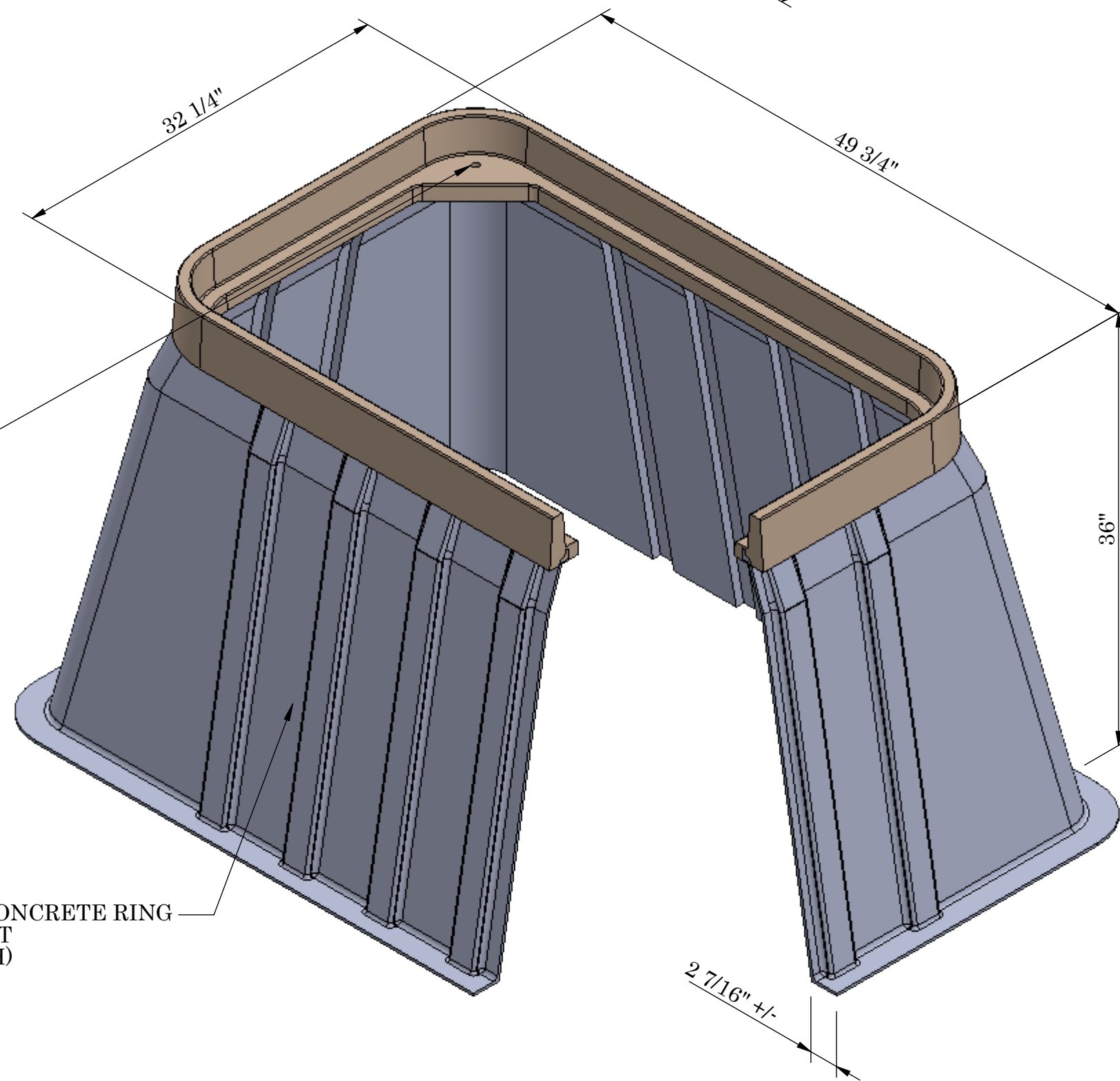
ISOMETRIC VIEW
