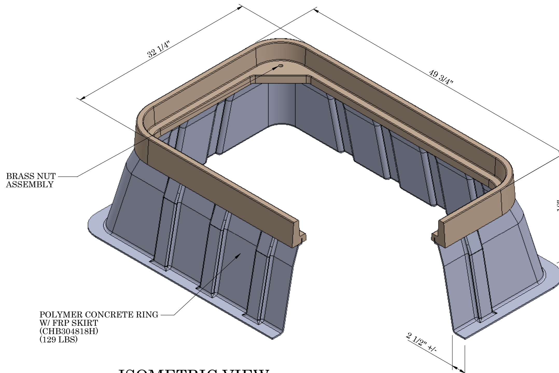
ISOMETRIC VIEW
