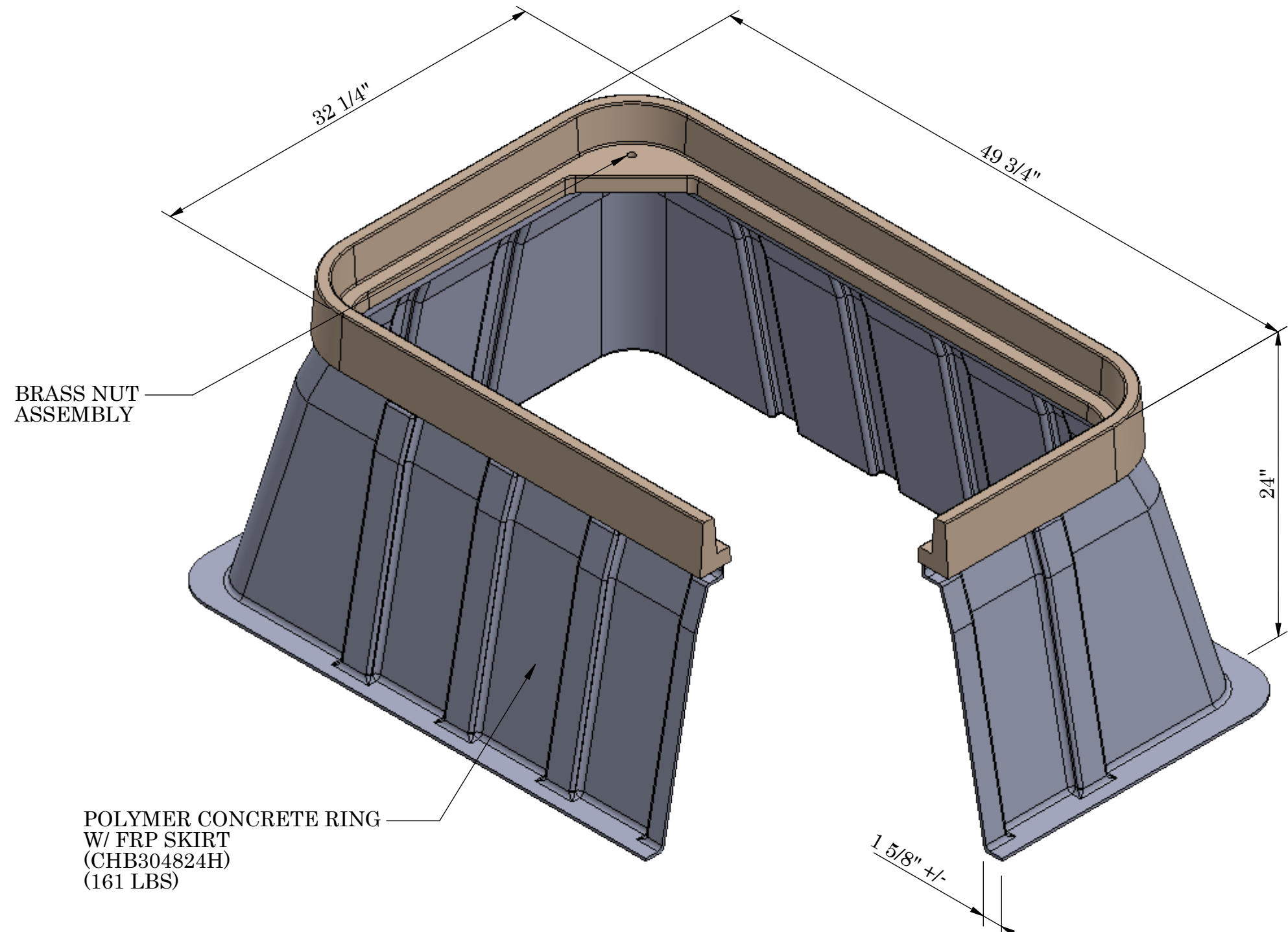
ISOMETRIC VIEW
