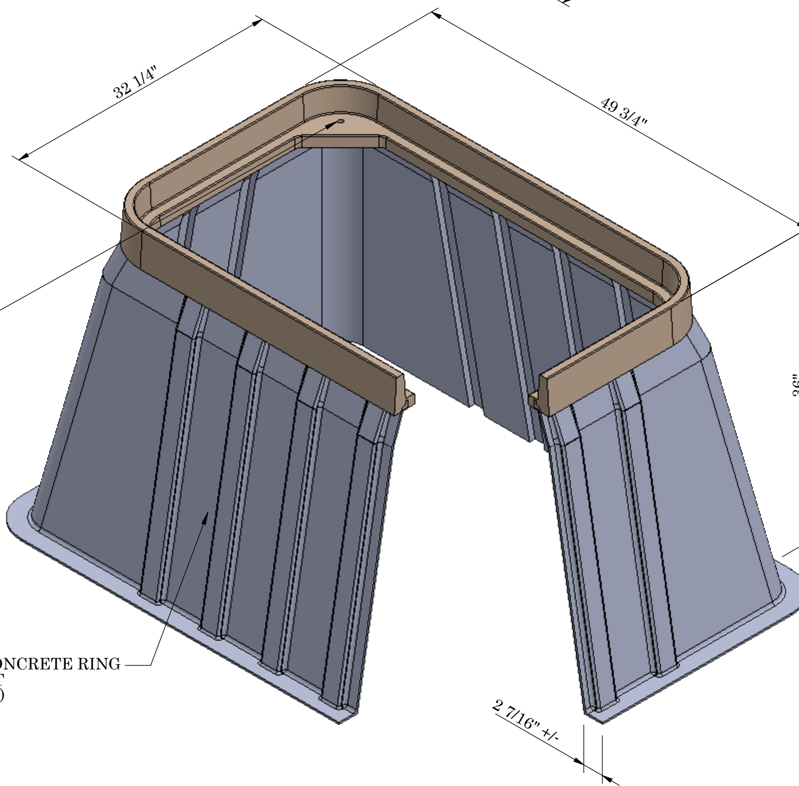
ISOMETRIC VIEW
