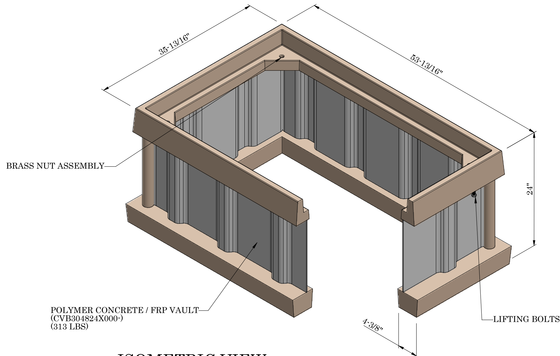
ISOMETRIC VIEW
