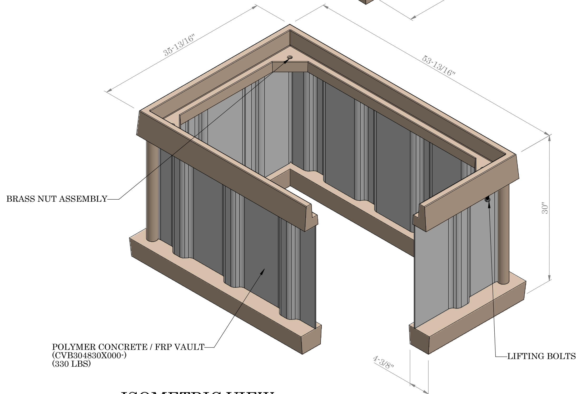
ISOMETRIC VIEW
