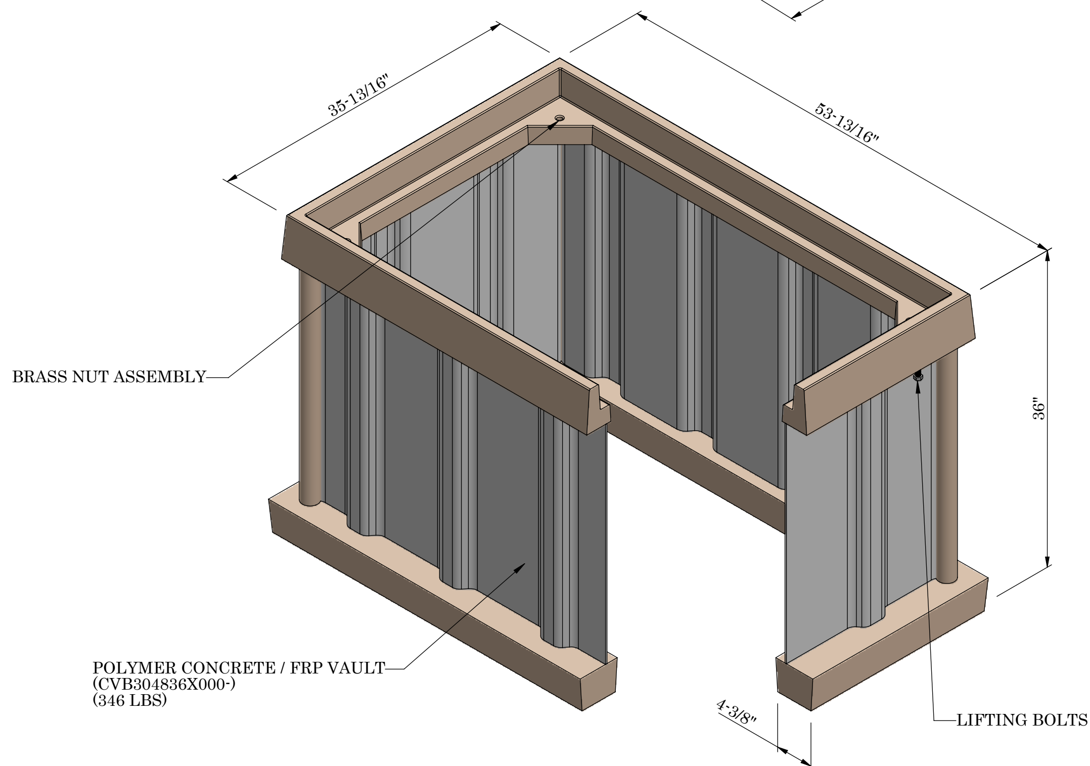
ISOMETRIC VIEW
