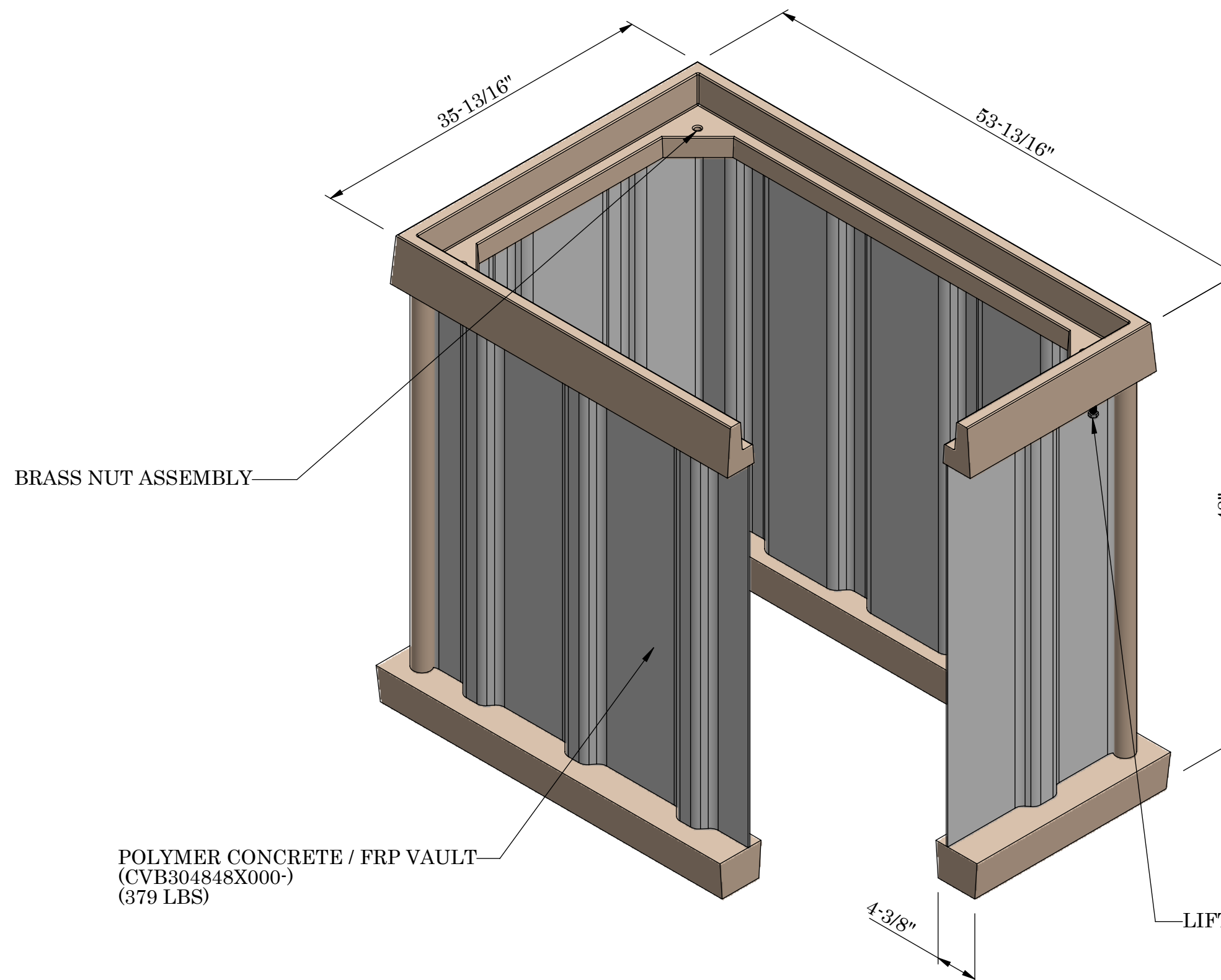
ISOMETRIC VIEW
