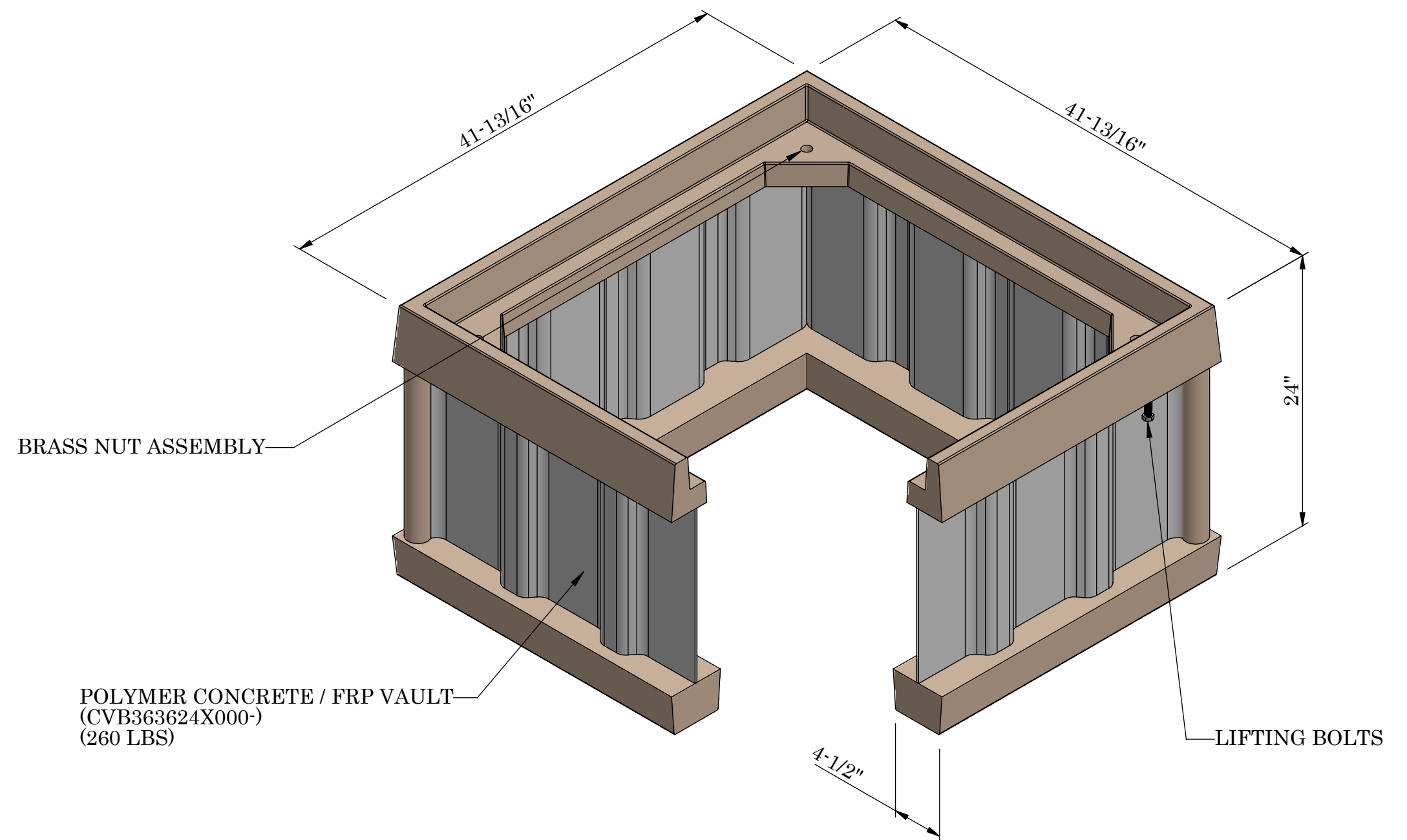
ISOMETRIC VIEW
