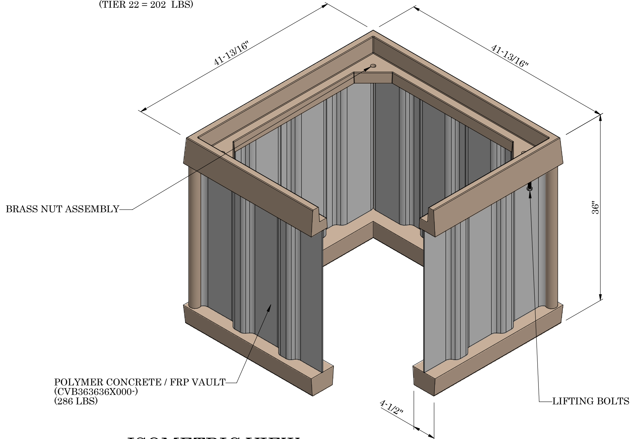
ISOMETRIC VIEW
