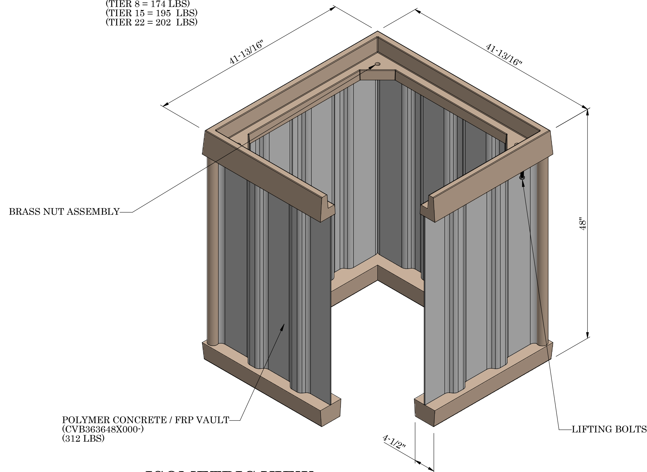
ISOMETRIC VIEW
