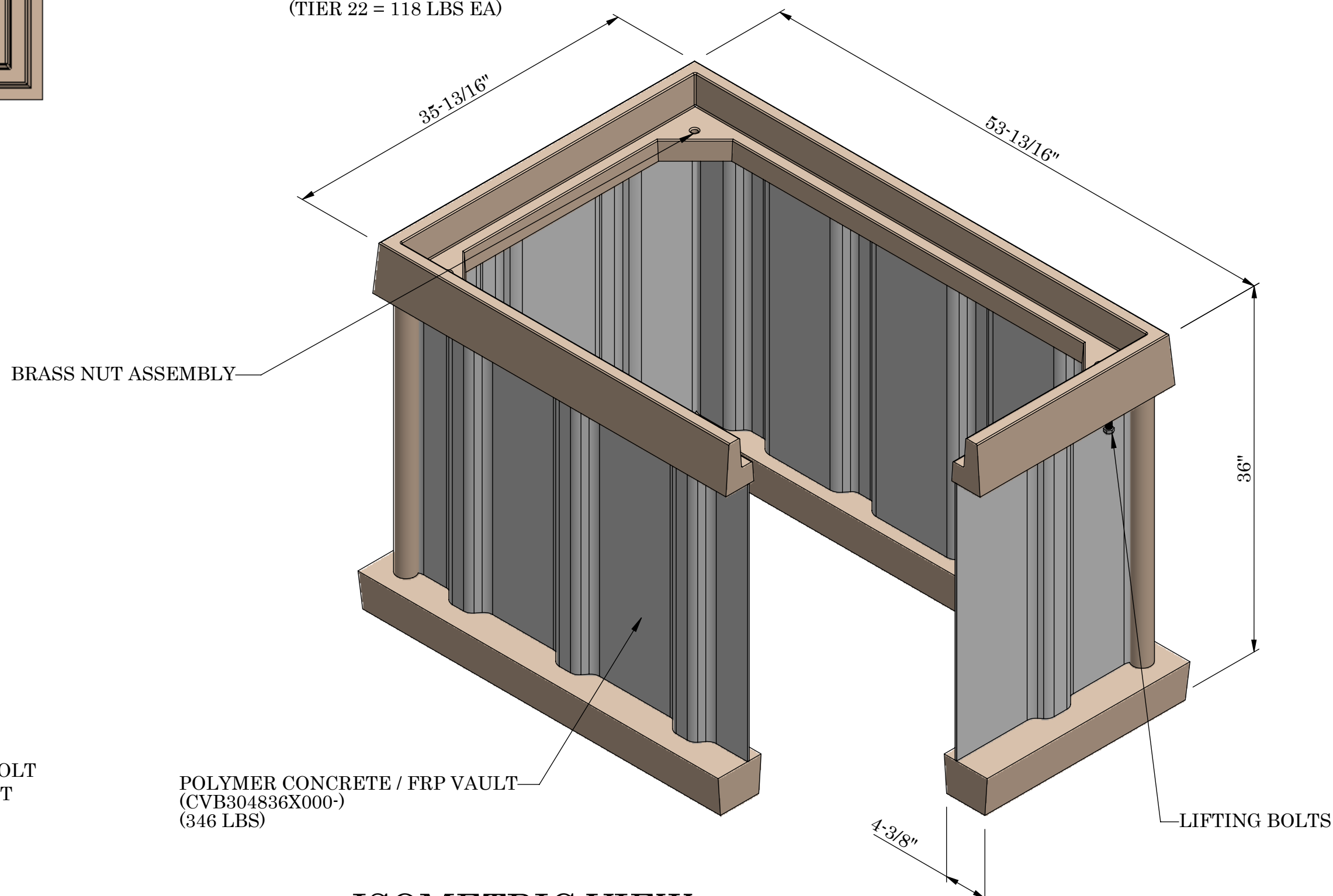
ISOMETRIC VIEW
