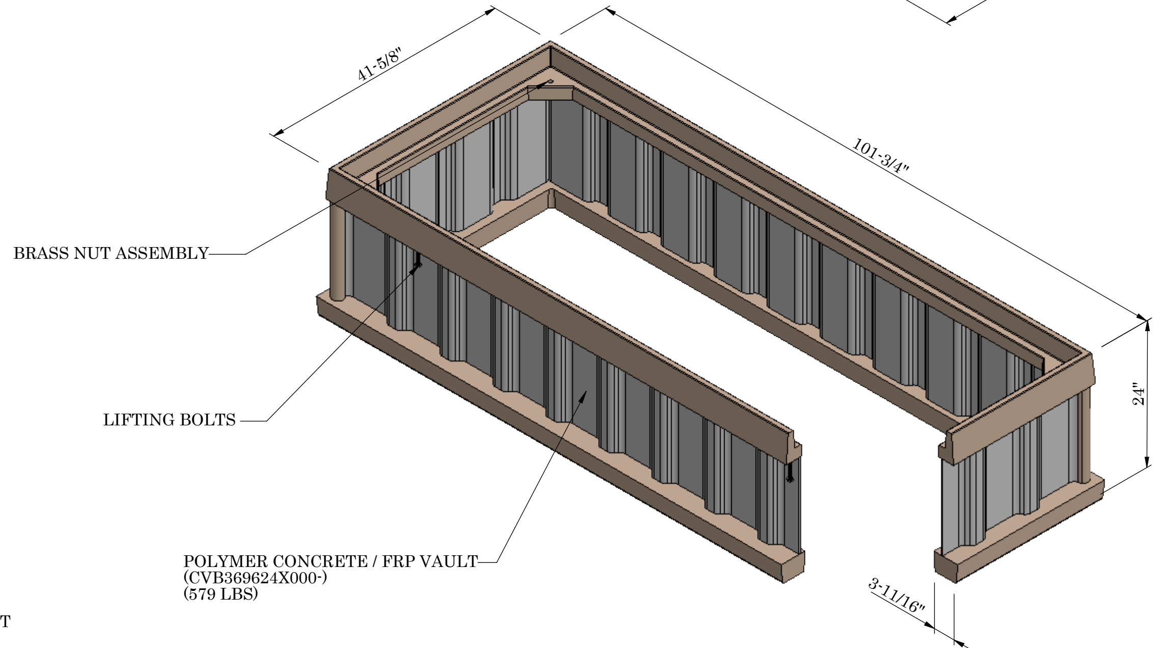
ISOMETRIC VIEW
