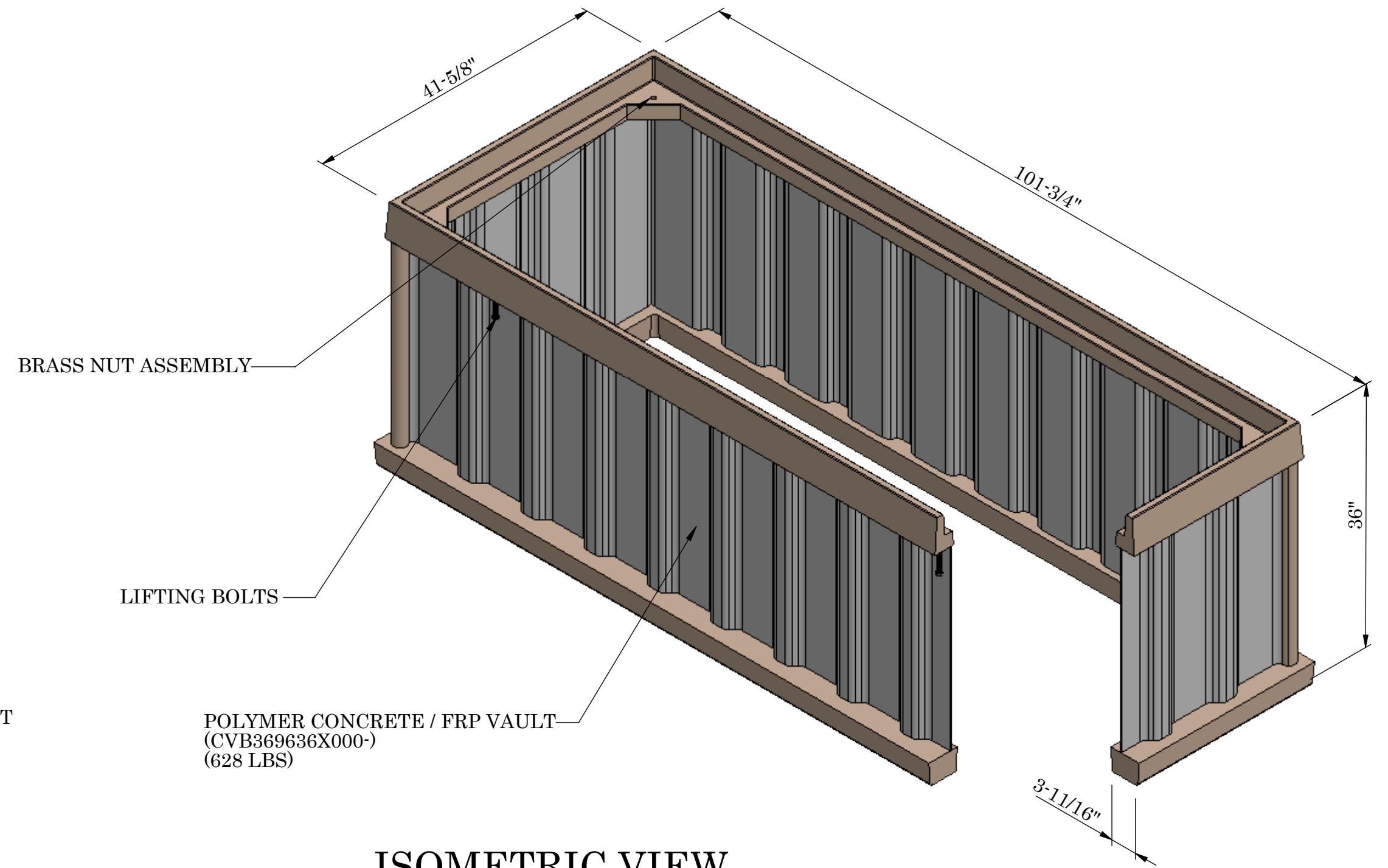
ISOMETRIC VIEW
