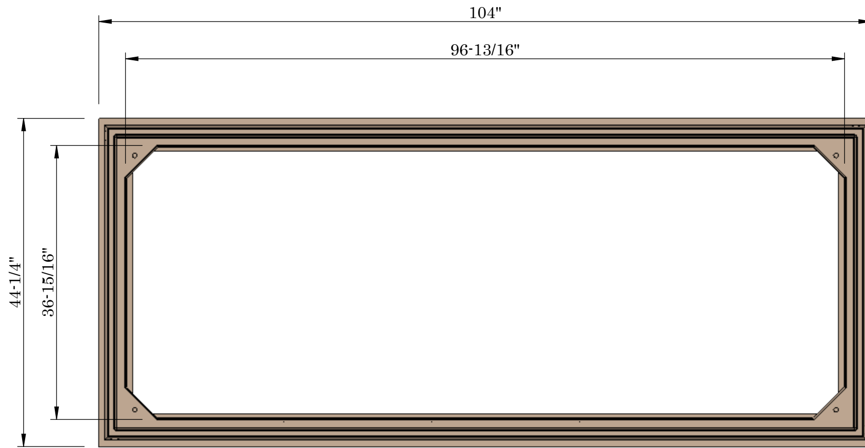
TOP VIEW OF BOX
