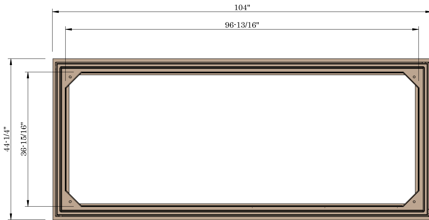
TOP VIEW OF BOX
