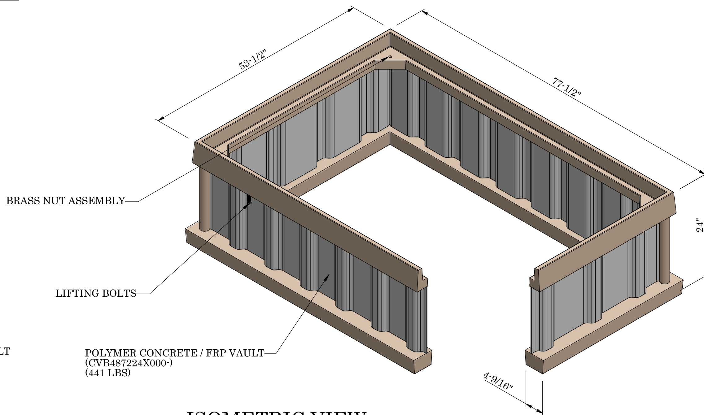
ISOMETRIC VIEW
