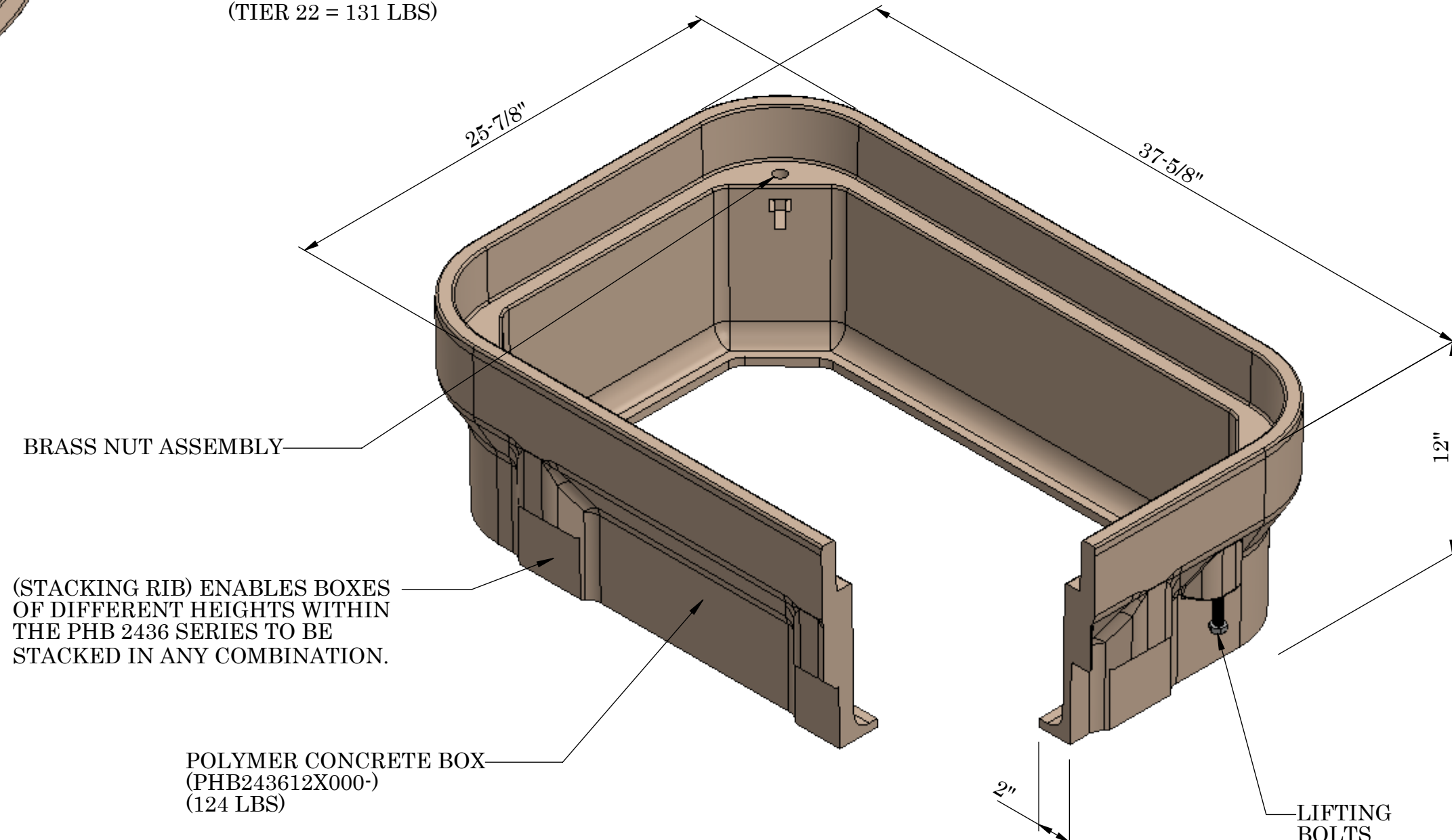
ISOMETRIC VIEW
