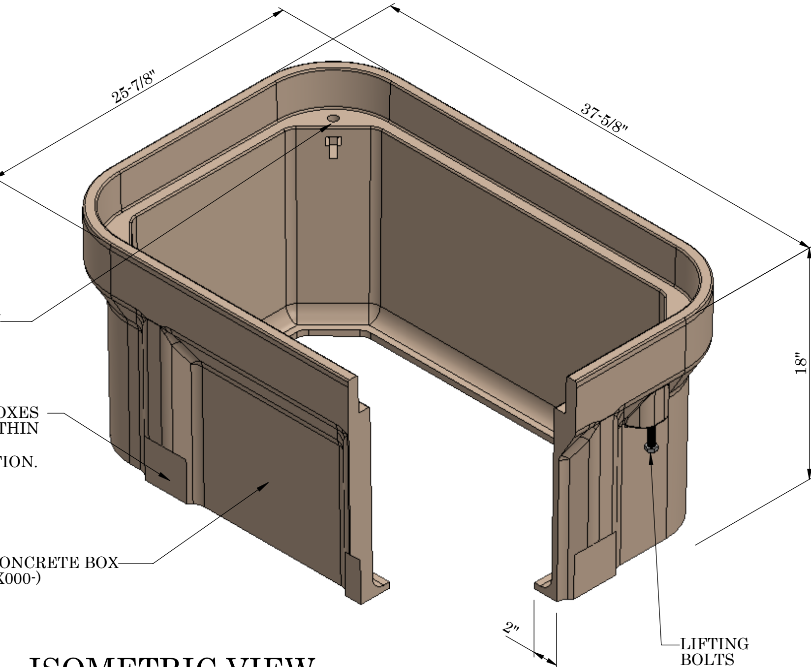
ISOMETRIC VIEW
