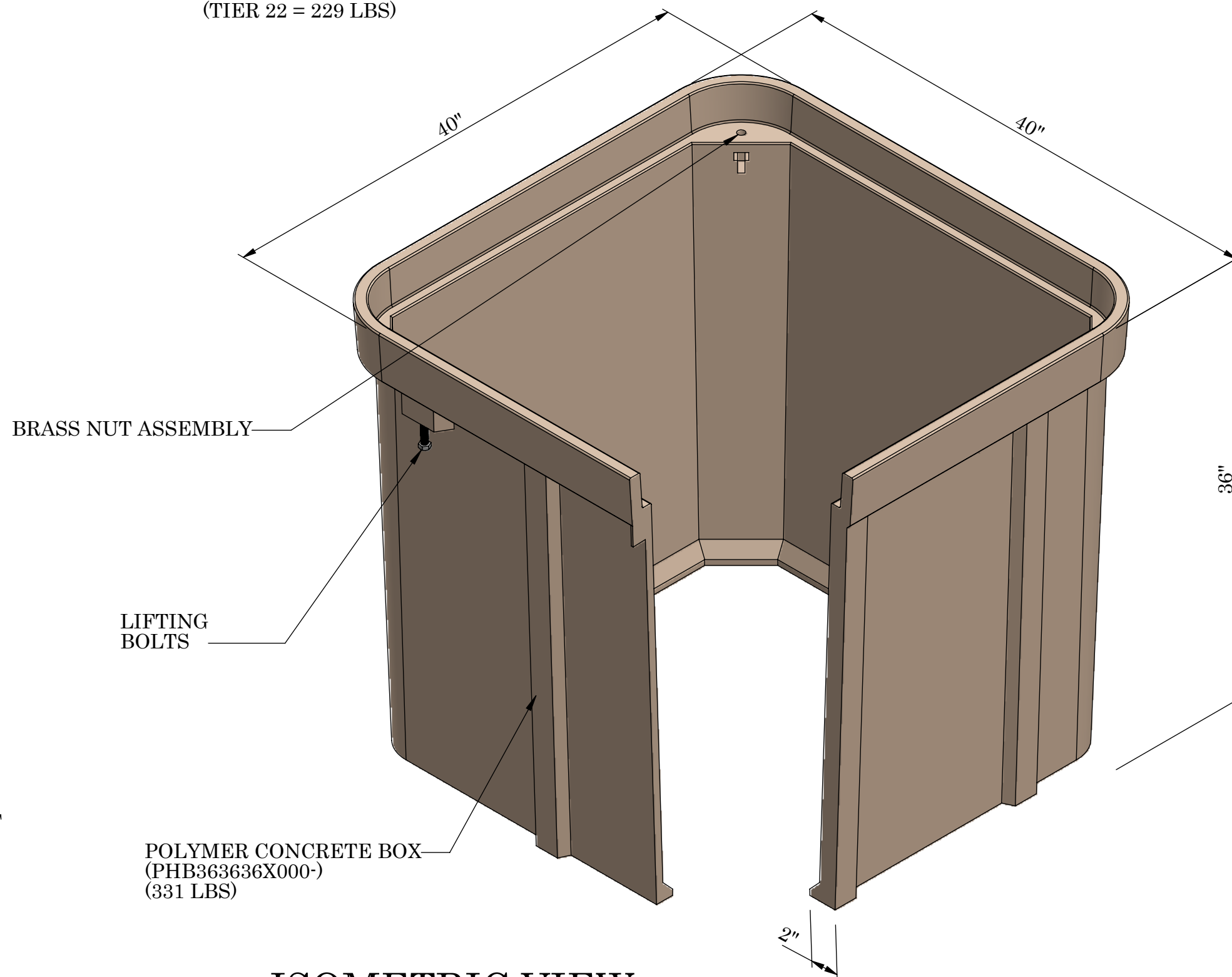
ISOMETRIC VIEW
