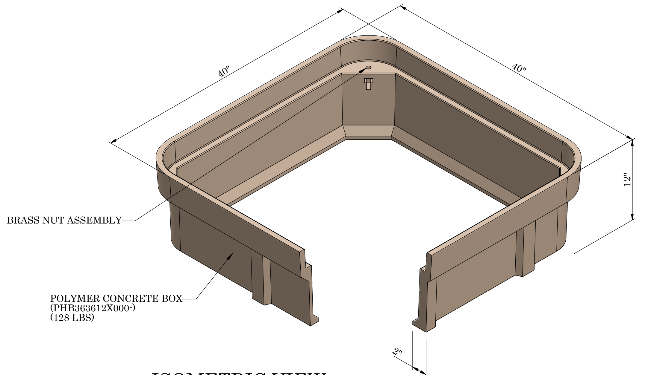
ISOMETRIC VIEW
