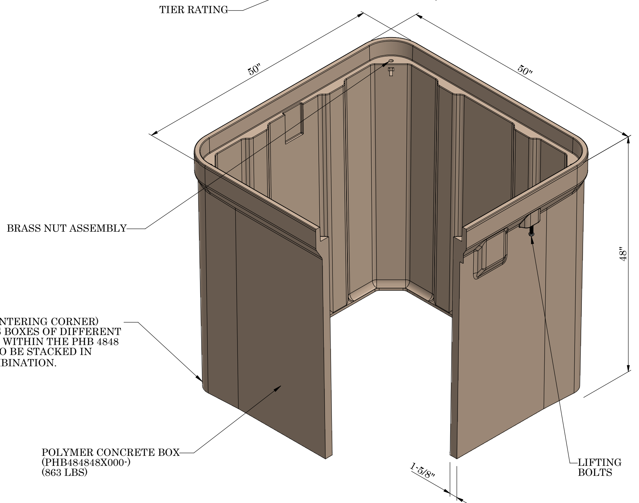
ISOMETRIC VIEW
