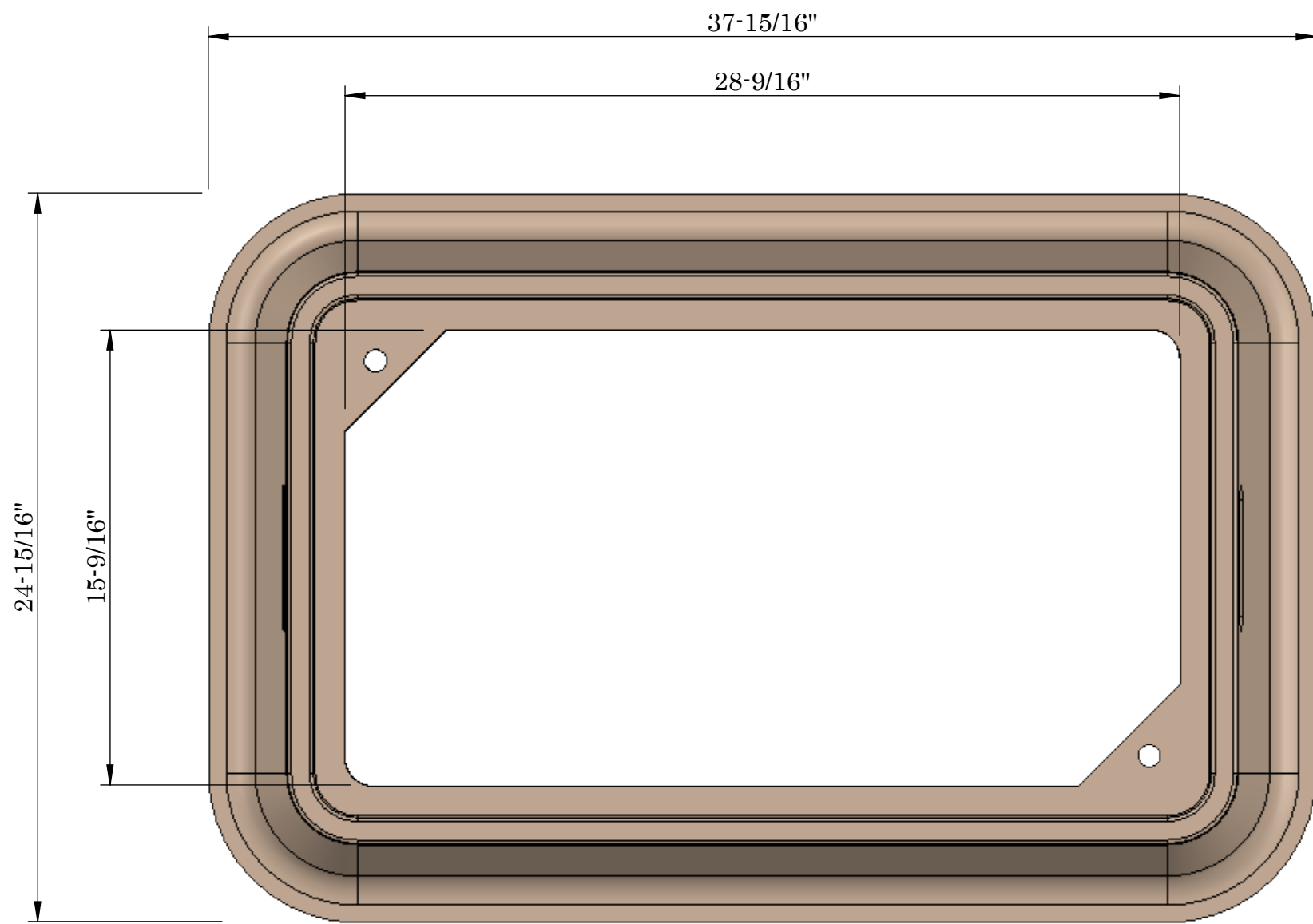
TOP VIEW OF BOX
